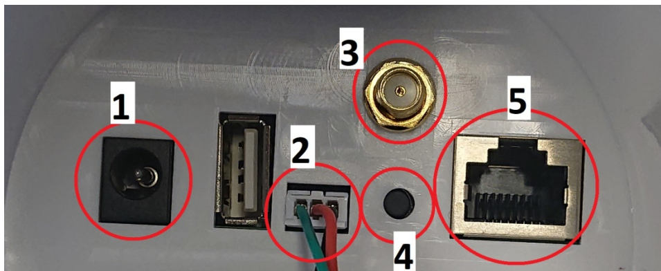
Figure 5: Ports on the gateway
